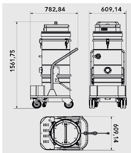
3 motores By-pass
